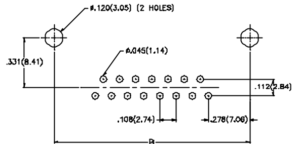
PCB LAYOUT REFERENCE
