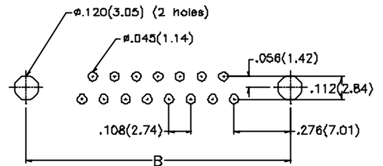
PCB LAYOUT REFERENCE
